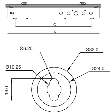
Mounting Hole Details
